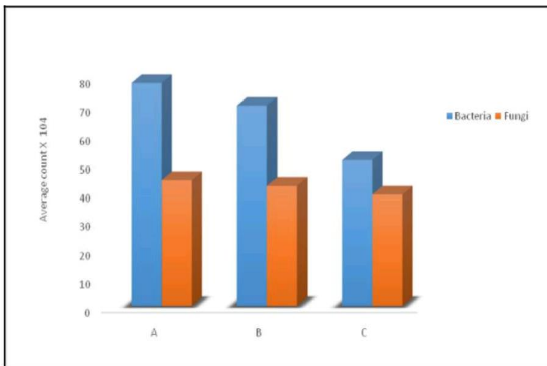
Figure 1 Bacterial and fungal counts at the impacted soil, un-impacted soil and cassava effluent (A Impacted soil, B - Un-impacted soil and C - Cassava effluent)
