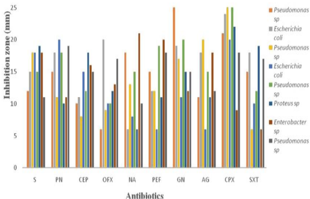
Figure 2 The sensitivity of different gram negative organisms and antibiotics
