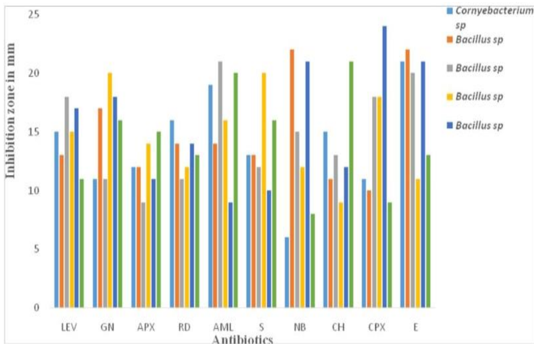
Figure 3 The sensitivity of different gram positive organisms and antibiotics
